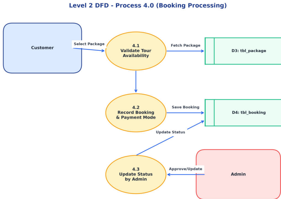
Figure 5.4: Level 2 Data Flow Diagram for Booking Sub-processes
