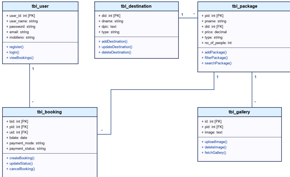
Figure 5.6: UML Class Diagram for AtlasGo Domain Model
