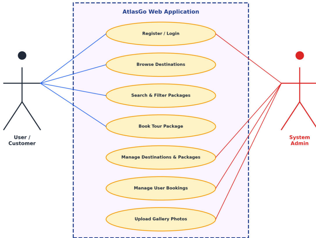
Figure 5.5: UML Use Case Diagram for User and Admin Roles
