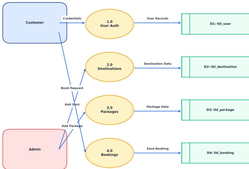
Figure 5.3: Level 1 Data Flow Diagram (DFD)
